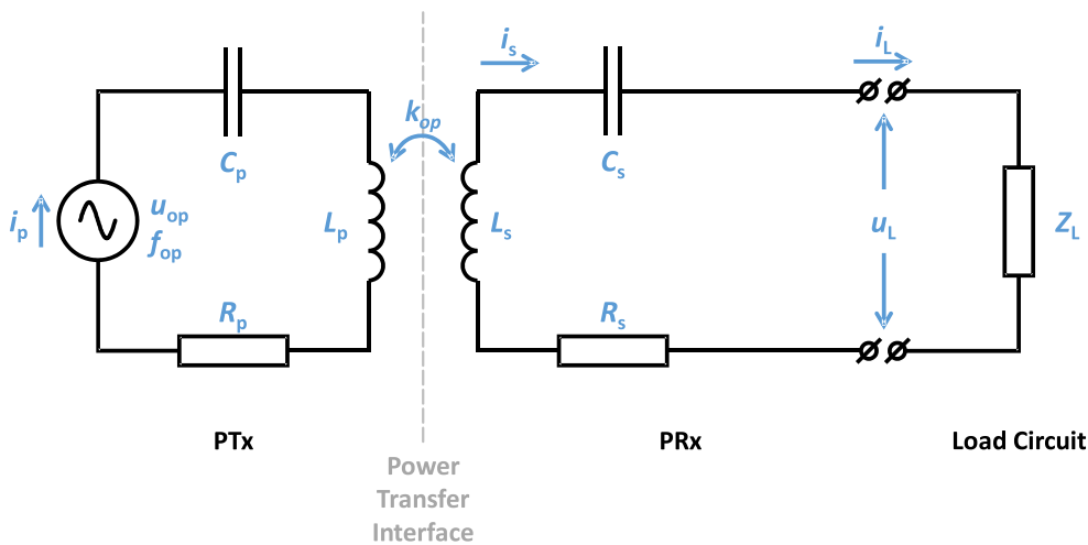
Figure 10. Simplified system model
