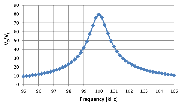
Figure 45. Q-factor measurement example
