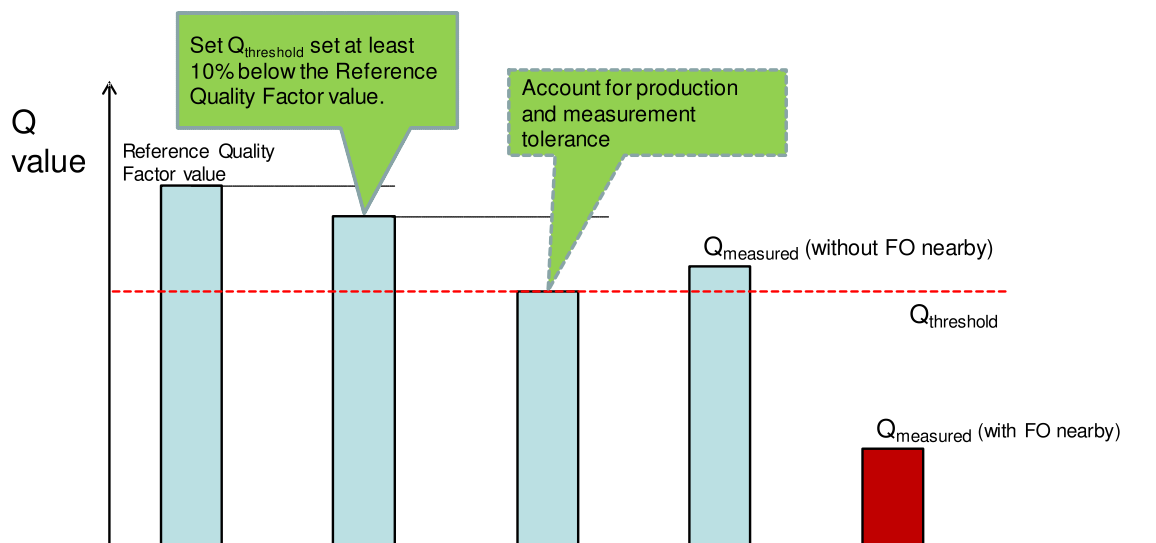
Figure 46. Quality factor threshold example
