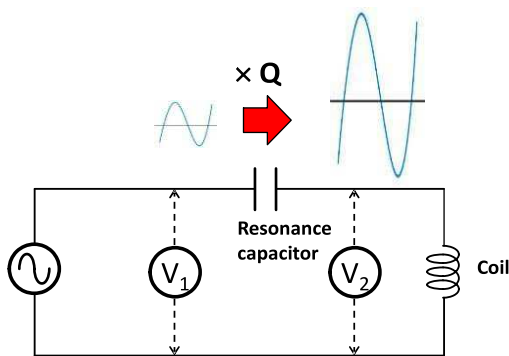
Figure 45. Q-factor measurement example
