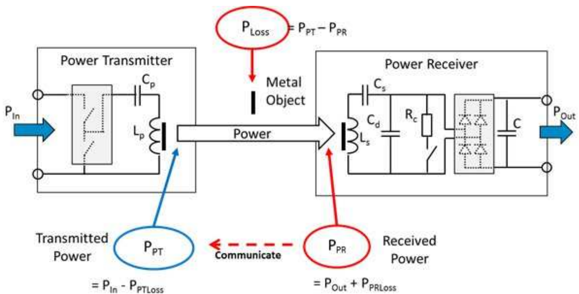
Figure 47. Power losses illustrated
