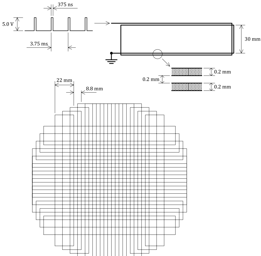
Figure 53. Detection Coil
