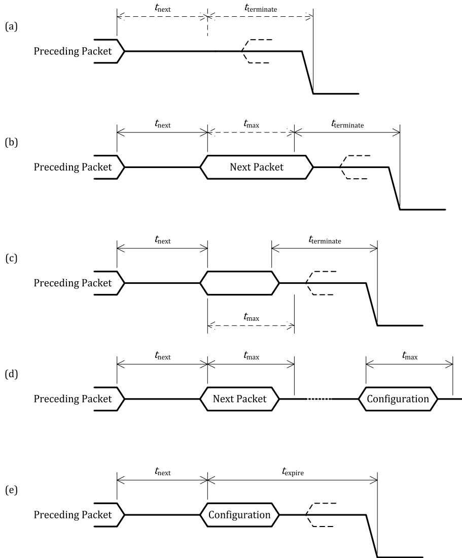
Figure 21. Power Transmitter timing in the identification & configuration phase (FOD extensions)
