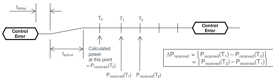
Figure 48. Computation of \Delta P_{\text{received}}
