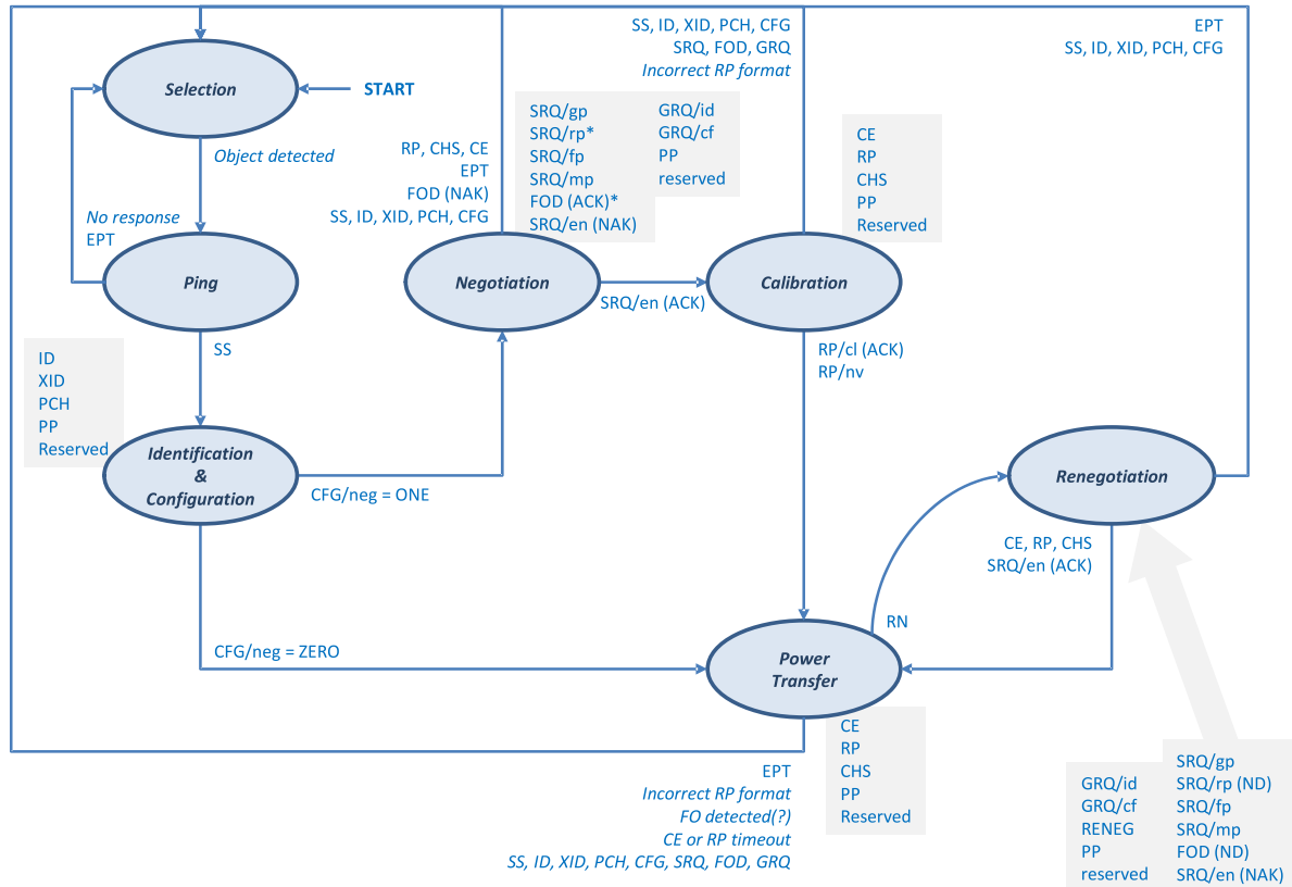
Figure 34. State diagram
