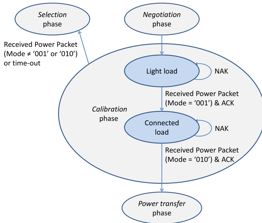
Figure 23. State diagram of the calibration phase
