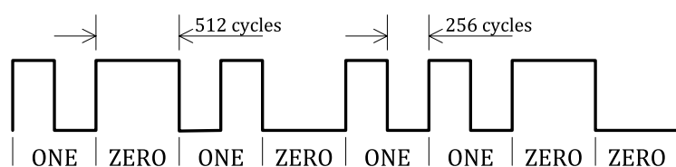
Figure 39. Example of differential bi-phase encoding
