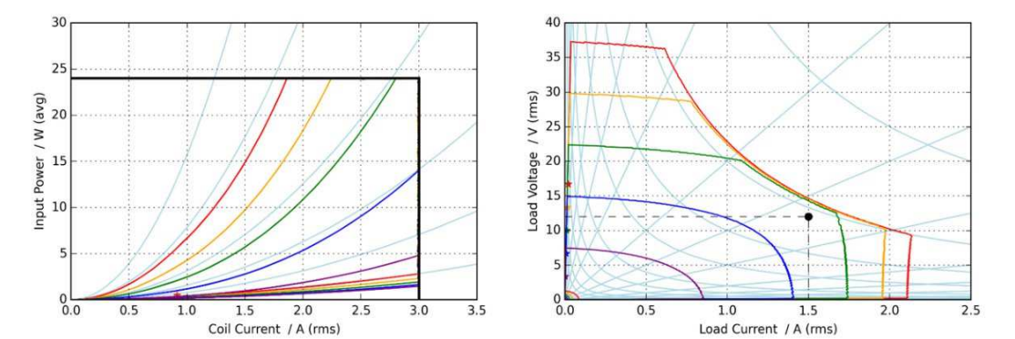
Figure 11. Operating space with a fixed-maximum Primary Coil current
